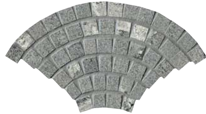
GNEISS GREY
