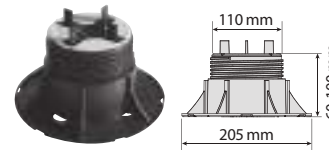
201008 V134 Supporto regolabile - Adjustable paving support mm 60/100
