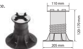
201005 V160 Supporto regolabile autolivellante Adjustable paving support self leveling head mm 120/170
